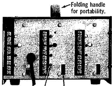
Typical rear view of CA-5, showing slot provides access to internal coding pins, connectors and line cord.
