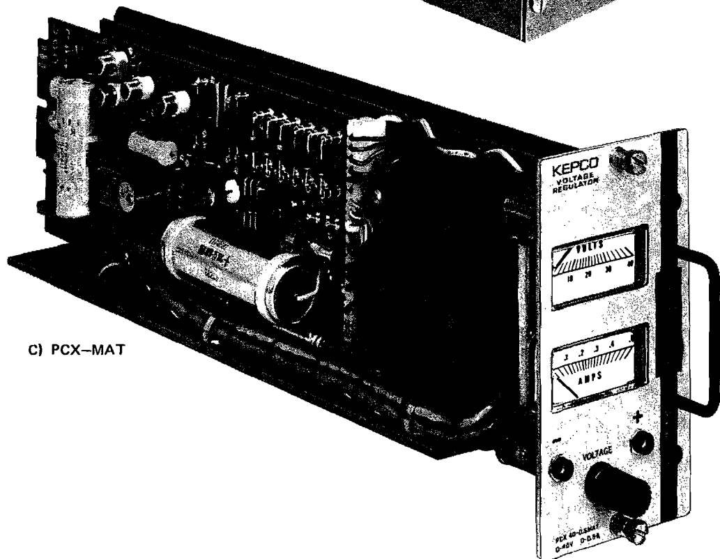
FIG. 1-1 KEPCO PCX AND PCX-MAT PLUG-IN MODULES
