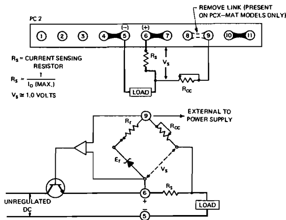
FIG. 3-8 CONNECTIONS FOR CONSTANT CURRENT OPERATION
