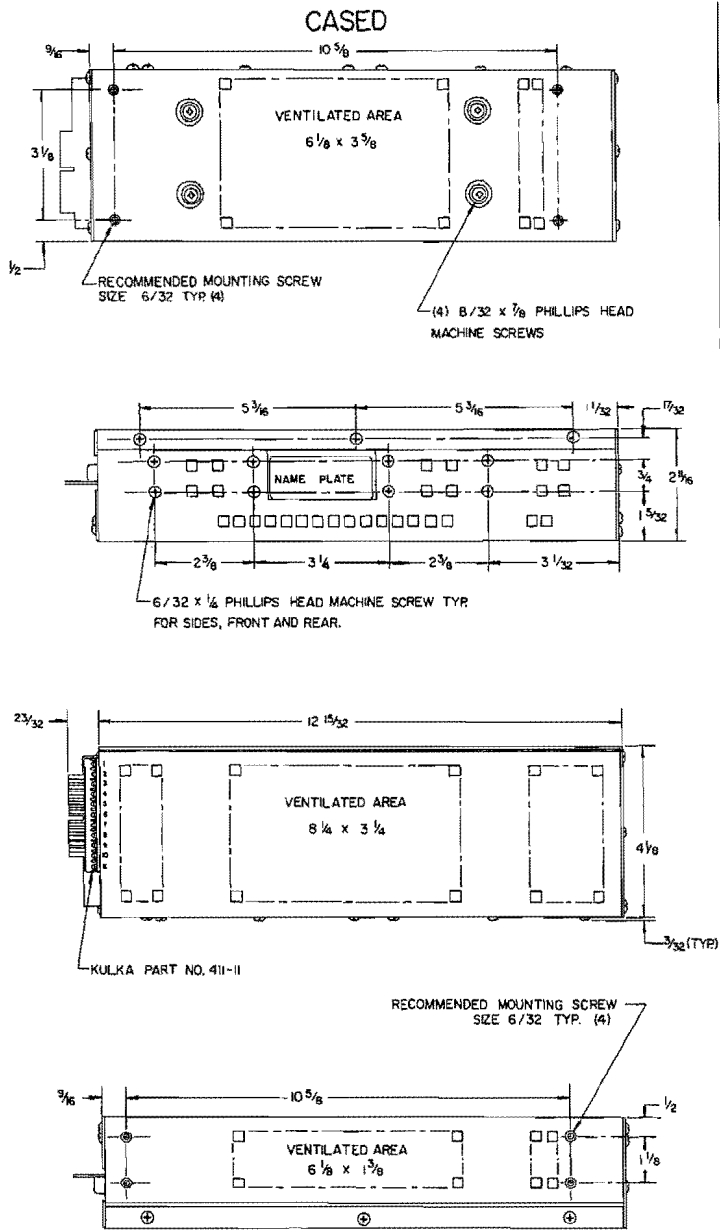
FIG. 1-3 MECHANICAL OUTLINE
