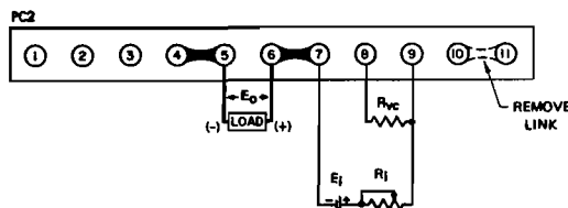
FIG. 3-10 CONNECTIONS FOR VOLTAGE PROGRAMMING
