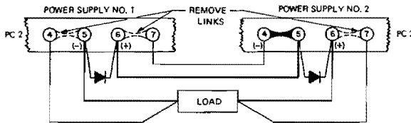
FIG. 3-11 SERIES CONNECTION OF PCX SUPPLIES
