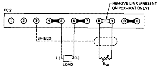
FIG. 3-7 CONNECTIONS FOR RESISTANCE PROGRAMMING
