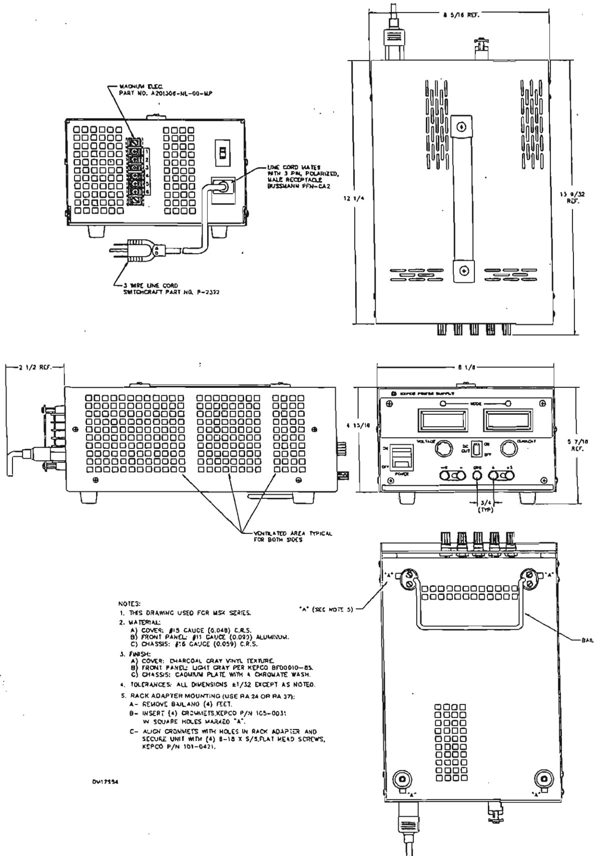
FIGURE 2-3. MECHANICAL OUTLINE
