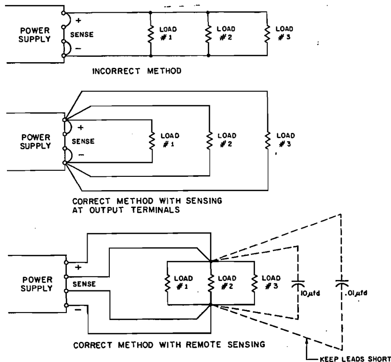
2-2 FIGURE 2-2 CORRECT AND INCORRECT METHODS OF CONNECTING MULTIPLE LOADS.
