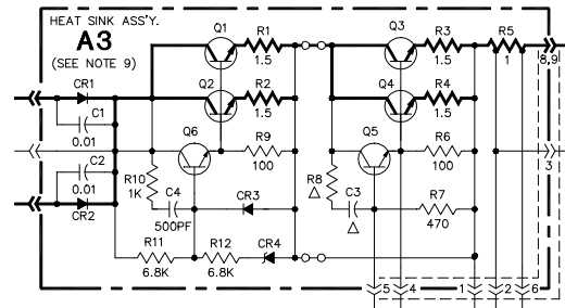
A3 HEAT SINK ASSEMBLY FOR MSK 125-1M ONLY
