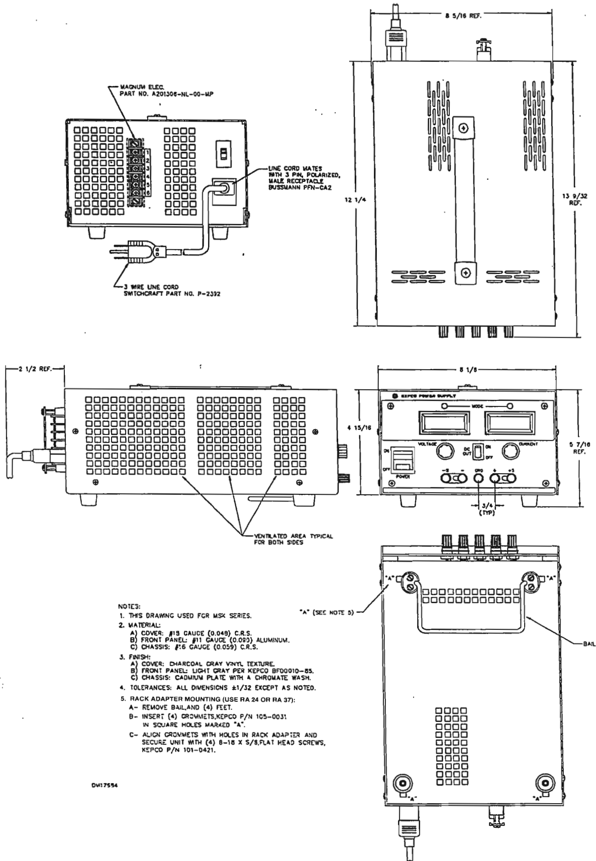
FIGURE 2-3. MECHANICAL OUTLINE
