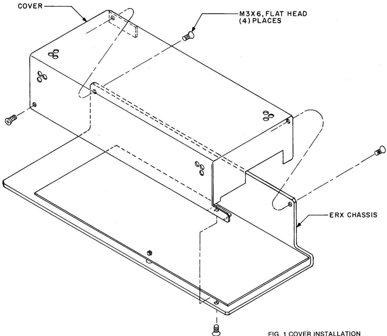
FIG. 1 COVER INSTALLATION
