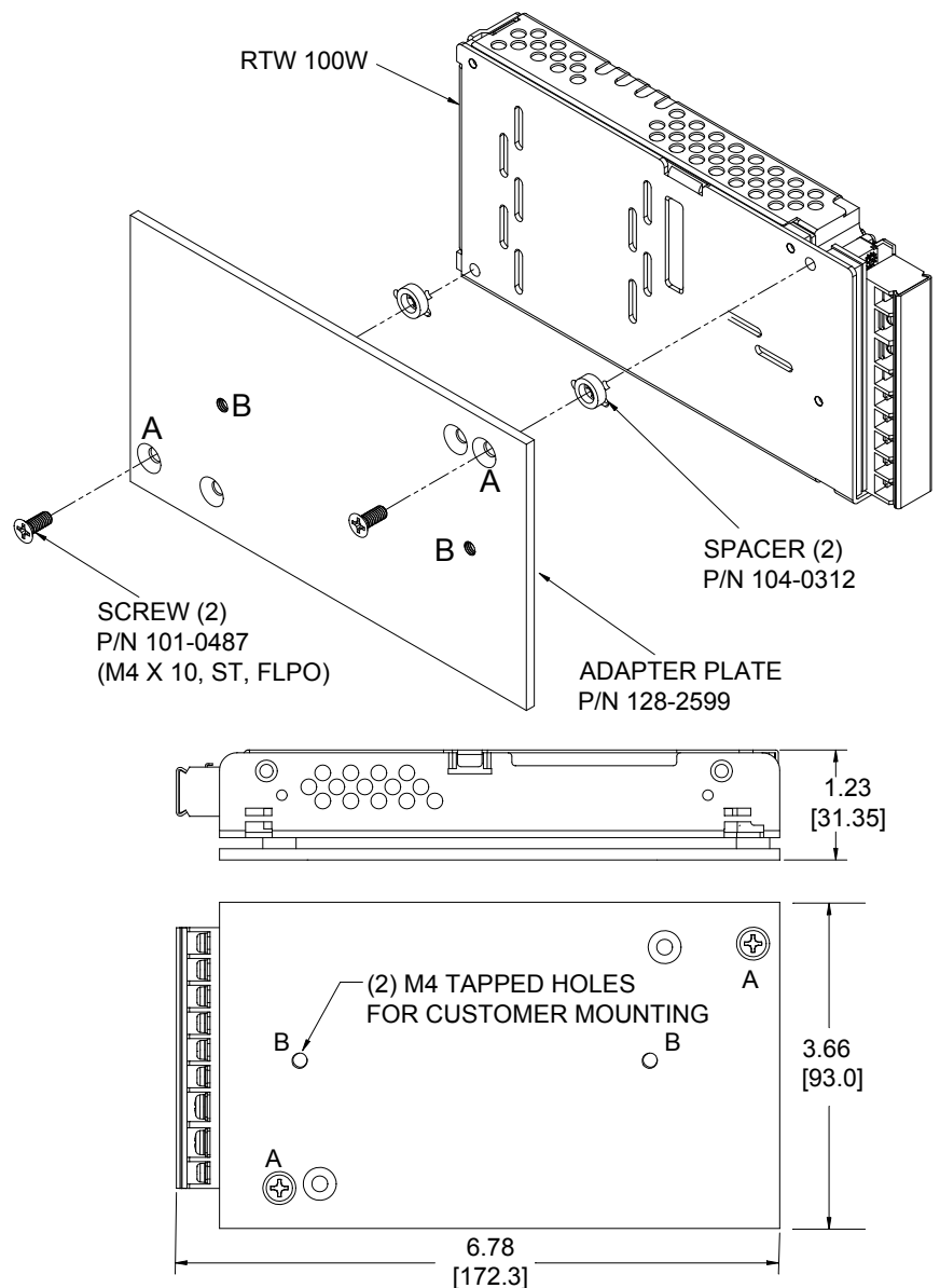
FIGURE 1. ADAPTER PLATE INSTALLATION
