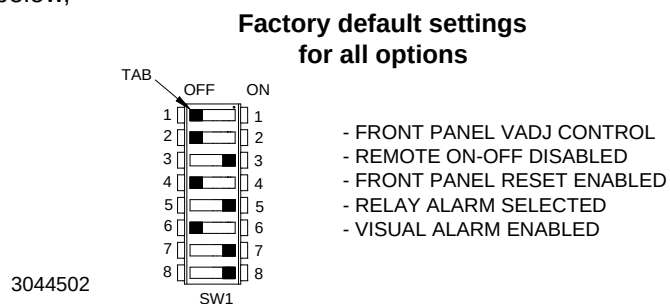
FIGURE 1. DIP SWITCH FACTORY DEFAULTS
