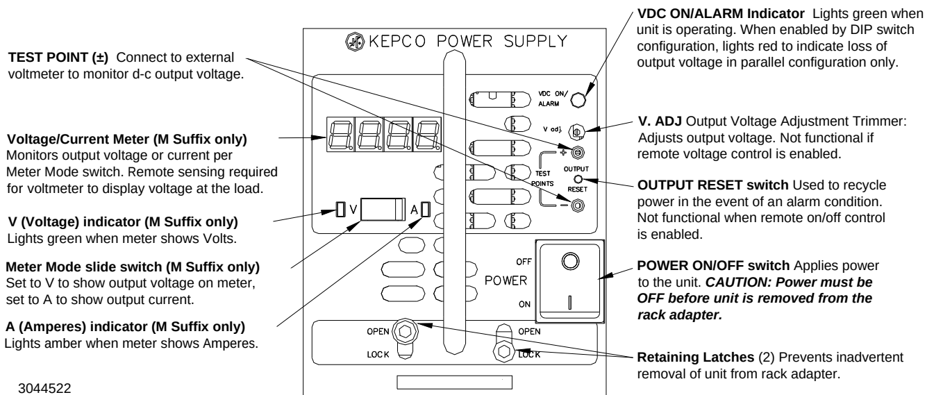
FIGURE 2. COMPONENT LOCATIONS
