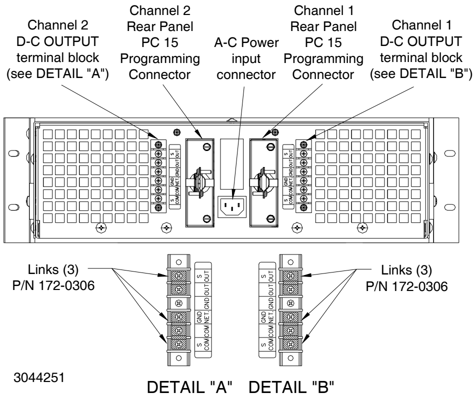
FIGURE 5. BOP 2X-D SERIES REAR PANEL TERMINATIONS
