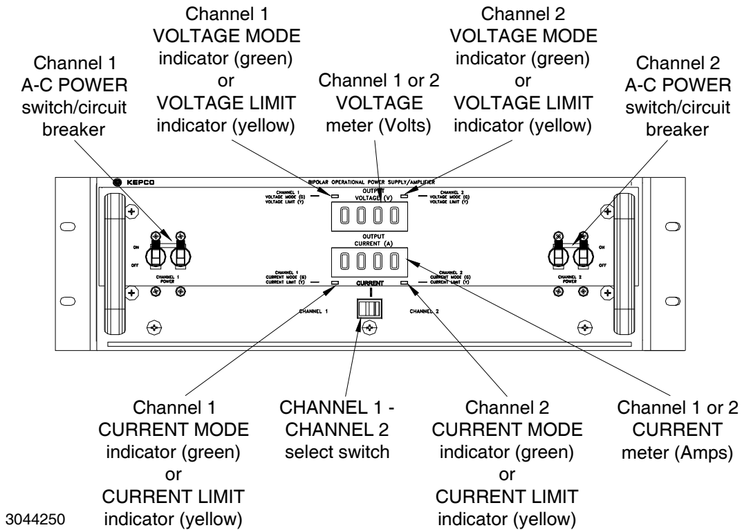
FIGURE 4. BOP 2X-D SERIES, FRONT PANEL CONTROLS AND INDICATORS
