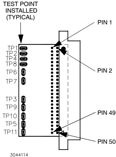
P/N 195-0121 PIN AND TEST POINT LOCATIONS
