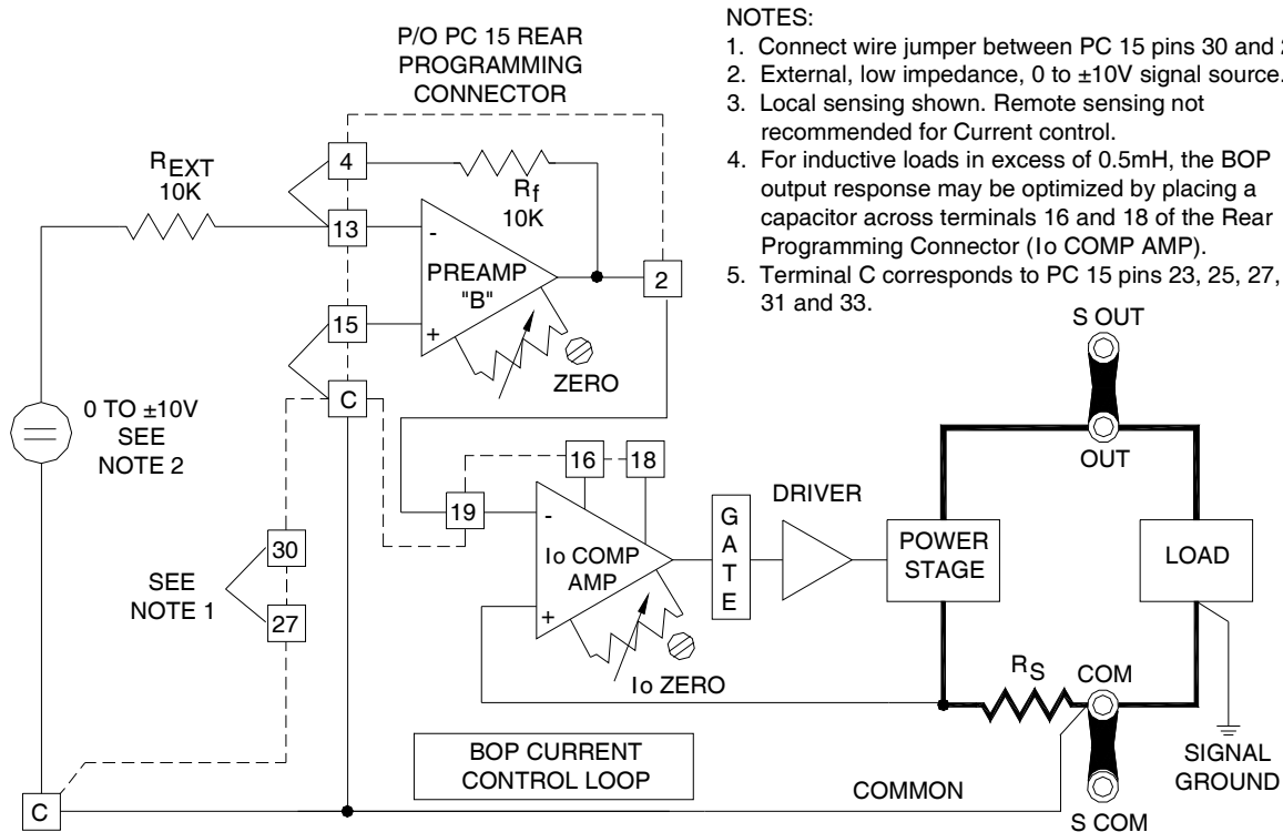
FIGURE 7. BOP 2X-D SERIES CHANNEL, OUTPUT CURRENT CONTROL
