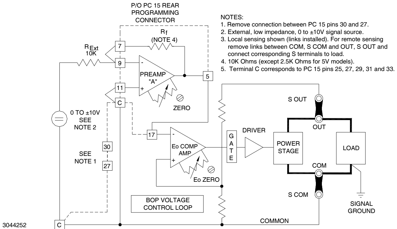
FIGURE 6. BOP 2X-D SERIES CHANNEL, OUTPUT VOLTAGE CONTROL
