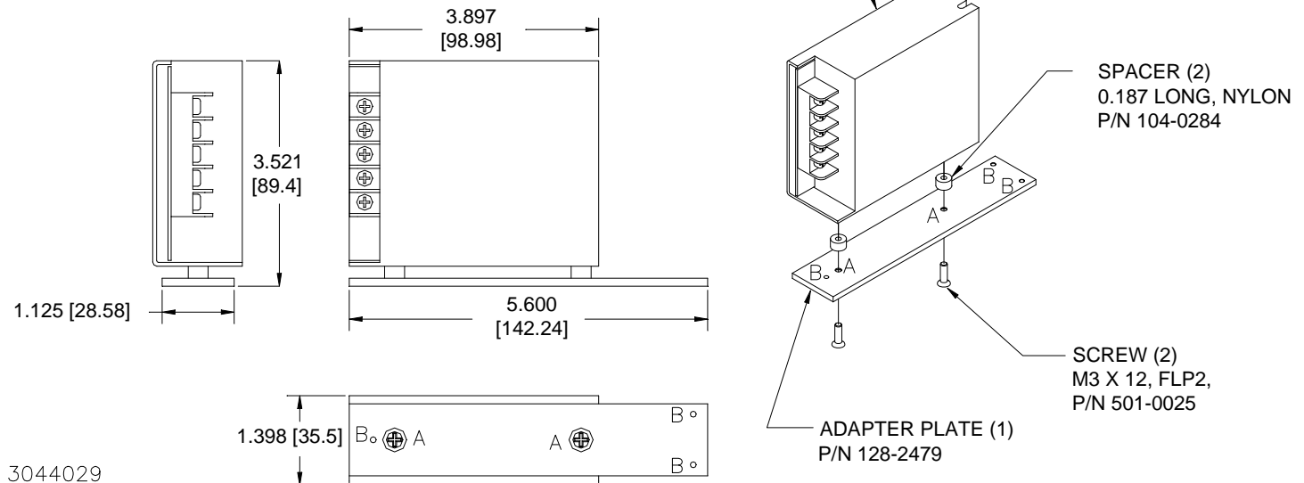
FIGURE 1. ADAPTER PLATE INSTALLATION
