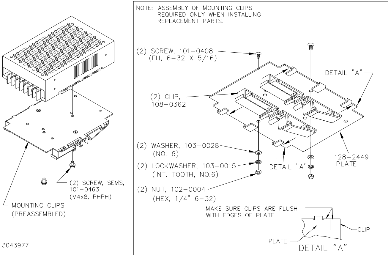
FIGURE 3. INSTALLATION OF KIT ON POWER SUPPLY
