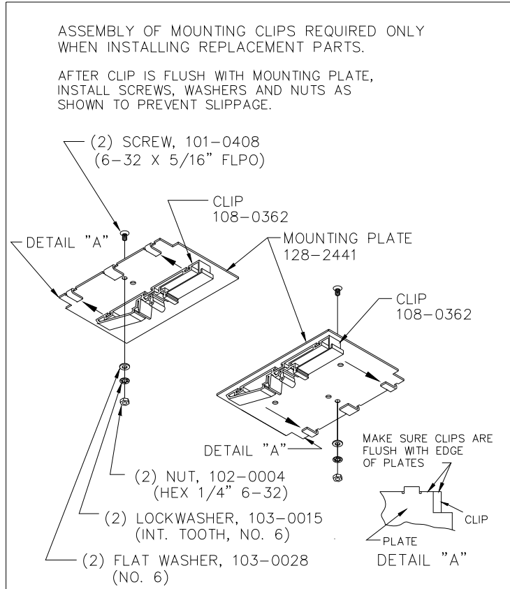
FIGURE 3. INSTALLATION OF KIT ON AE POWER SUPPLY
