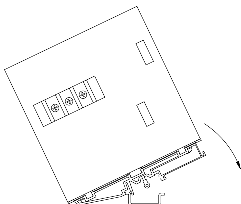
A — INSTALLATION
