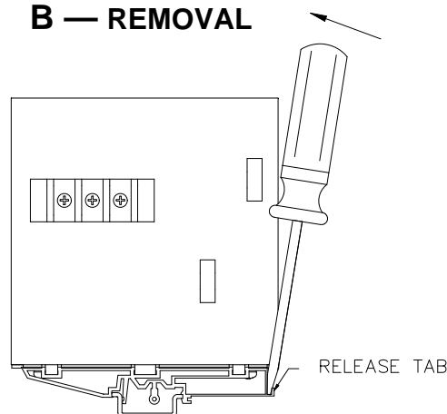
B — REMOVAL
