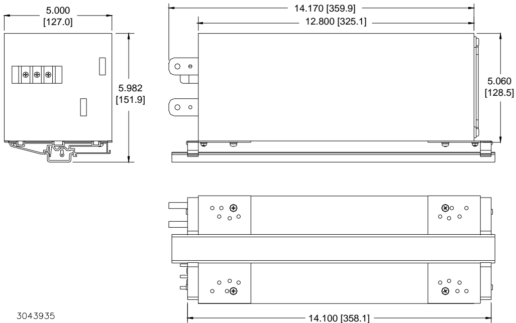
FIGURE 4. AE-3000 POWER SUPPLY WITH KIT INSTALLED, OUTLINE DIMENSIONS
