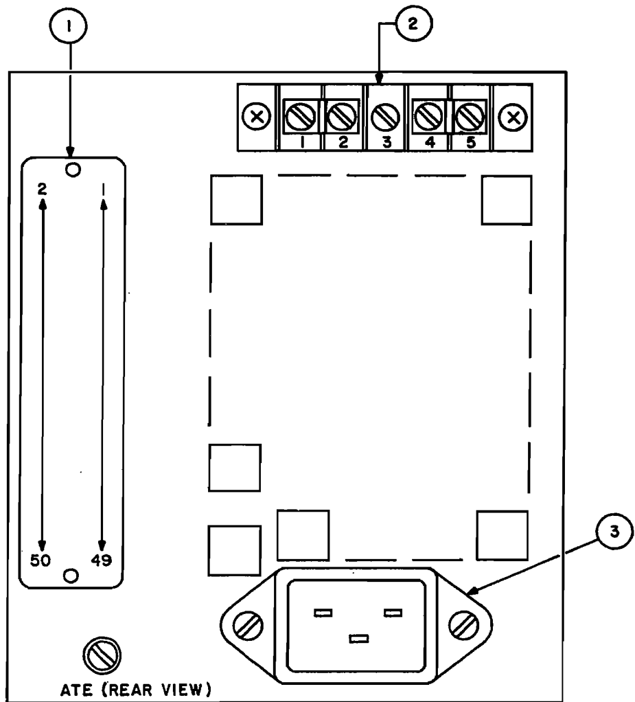
FIG. 2-3 TERMINATIONS, ATE 1/4 RACK GROUP, REAR.
