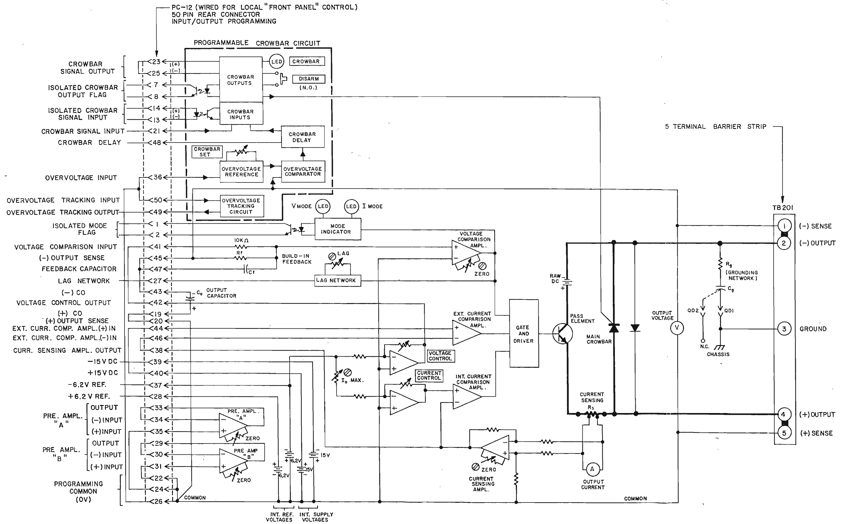
FIG. 3-32 ATE 1/4 RACK SIMPLIFIED SCHEMATIC DIAGRAM
