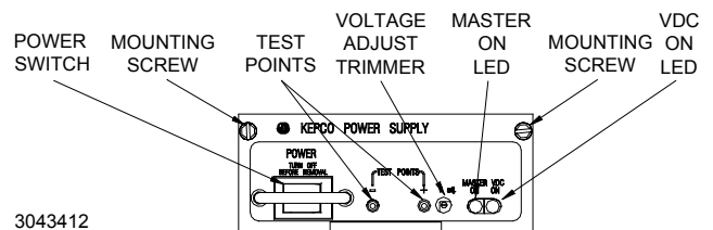
FIGURE 1. COMPONENT LOCATIONS
