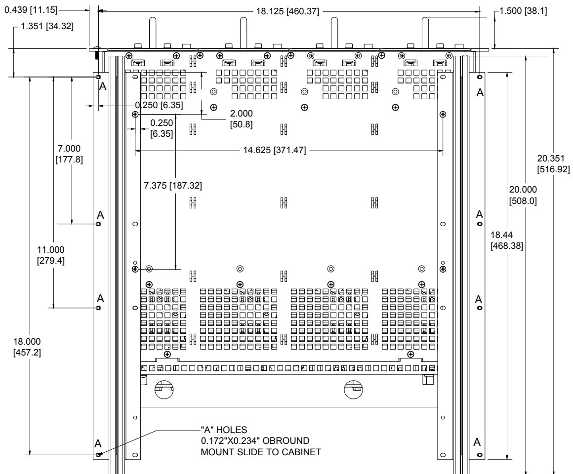
FIGURE 2. INSTALLING CHASSIS SLIDES ON RACK ADAPTER (FRONT VIEW)
