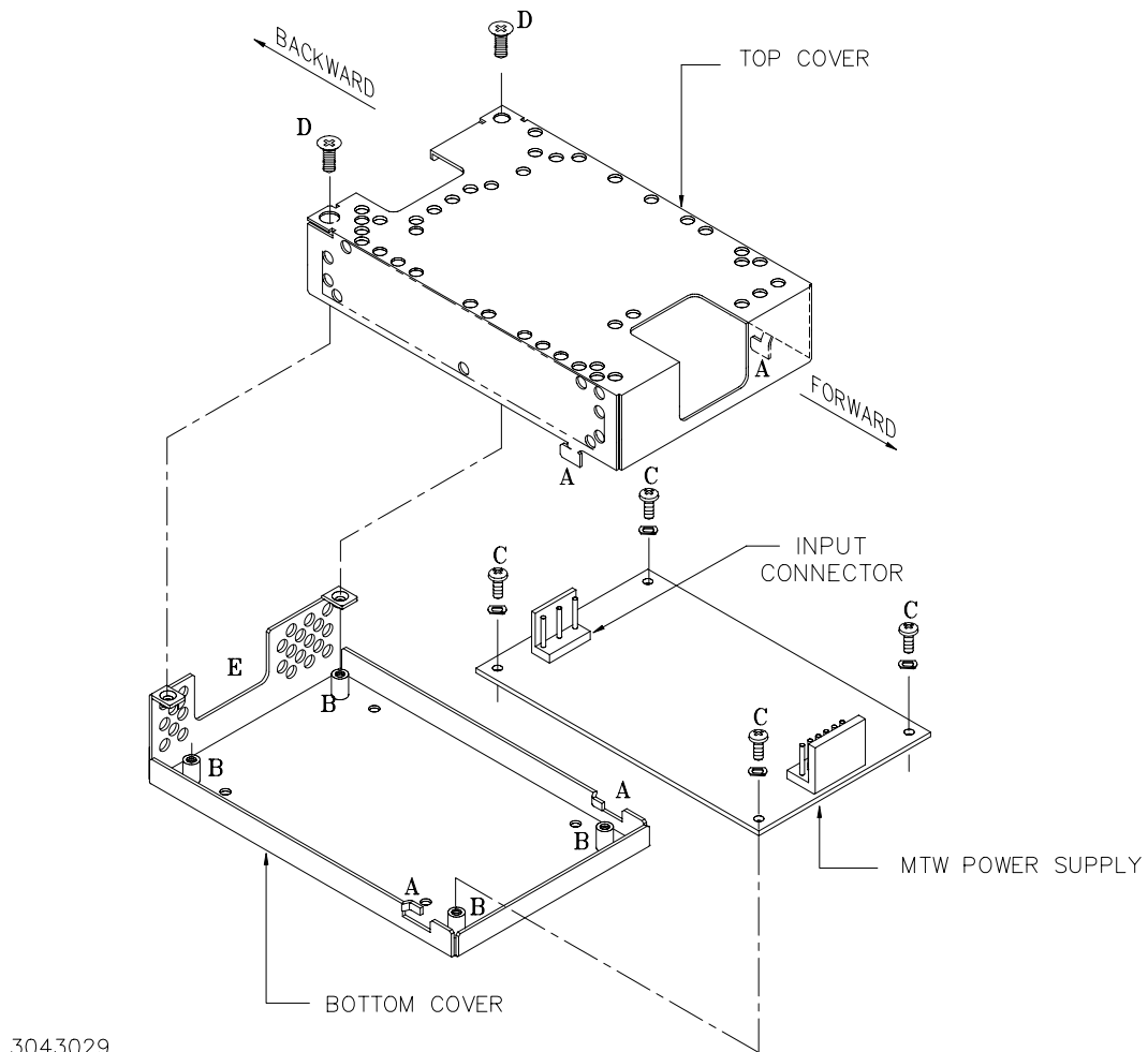
FIGURE 1. COVER INSTALLATION
