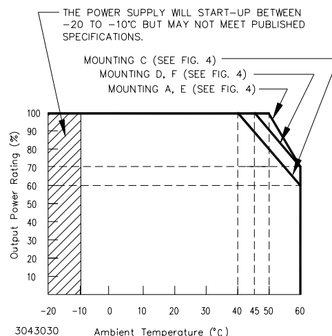
FIGURE 1. DERATING PLOT
