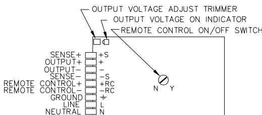
FIGURE 3. COMPONENT LOCATIONS
