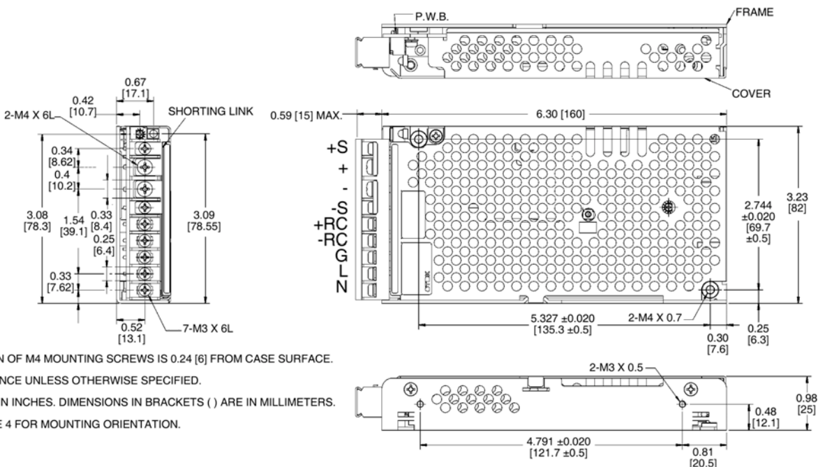
FIGURE 7. RTW 100W KC MODELS (WITH COVER) MECHANICAL OUTLINE DIAGRAM
