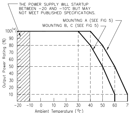
* MOUNTING A: AT INPUT VOLTAGE 85-90V, 100% IS DERATED TO 90%. MOUNTING B, C: AT INPUT VOLTAGE 85-90V, 100% IS DERATED TO 80%. AS INPUT VOLTAGE INCREASES FROM 90V TO 100V, OUTPUT POWER INCREASES LINEARLY FROM 80% AT 90V TO 100% AT 100V. 3043083
