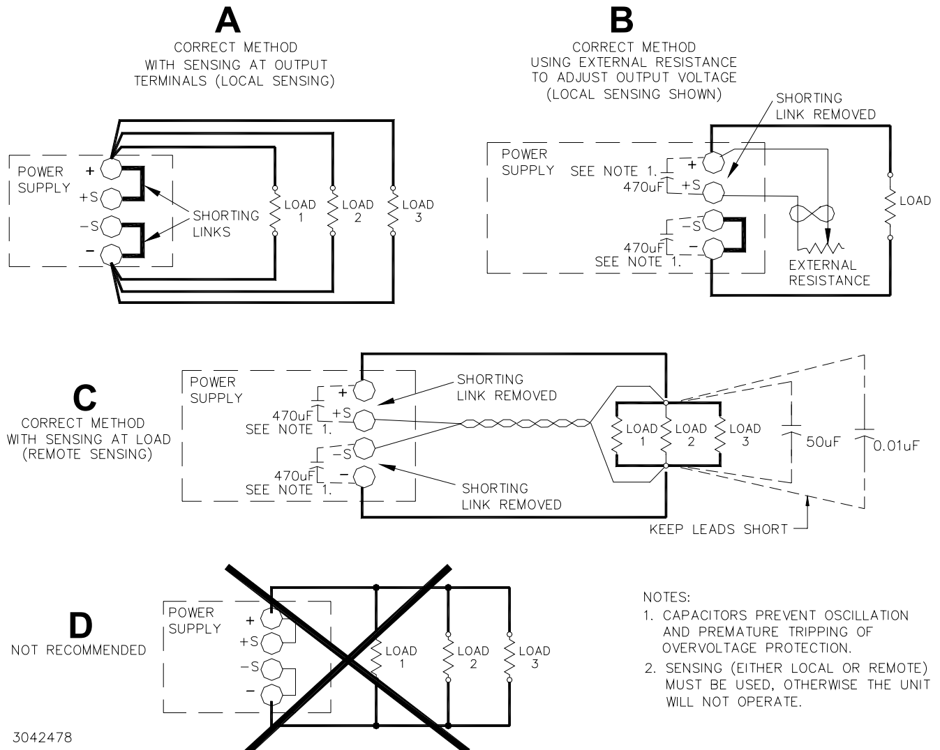
FIGURE 4. LOAD CONNECTIONS
