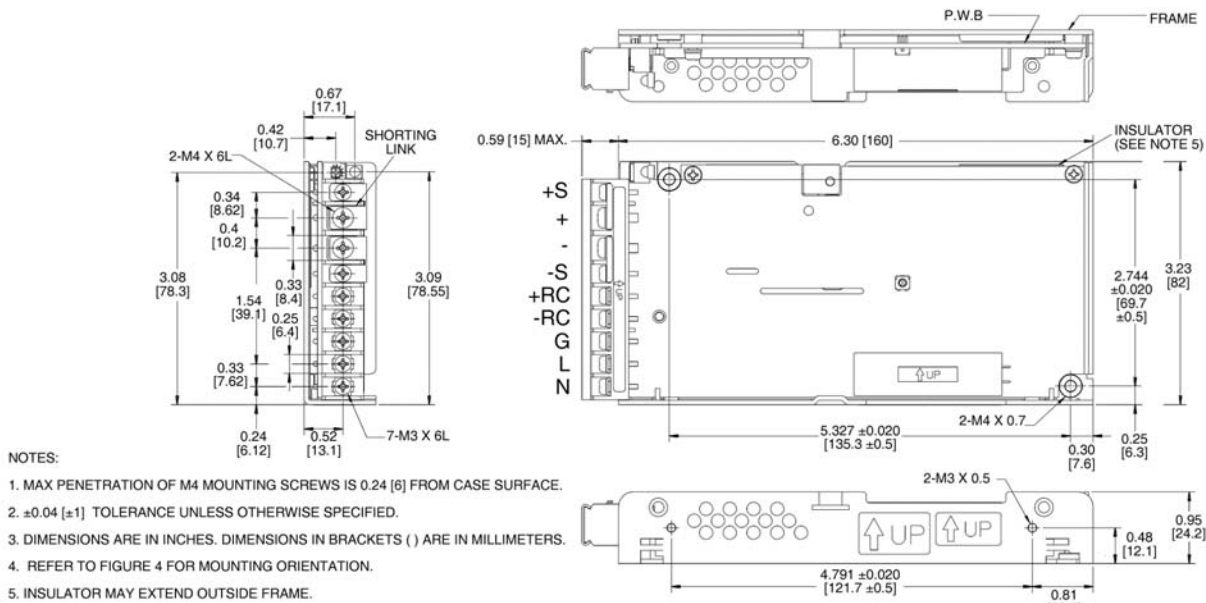
FIGURE 6. RTW 100W K MODELS (WITHOUT COVER) MECHANICAL OUTLINE DIAGRAM
