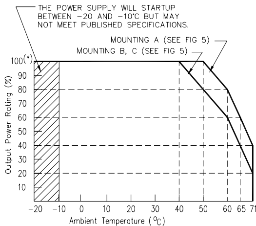
* AT INPUT VOLTAGE 85-90V, 100% IS DERATED TO 90%. 3042870
