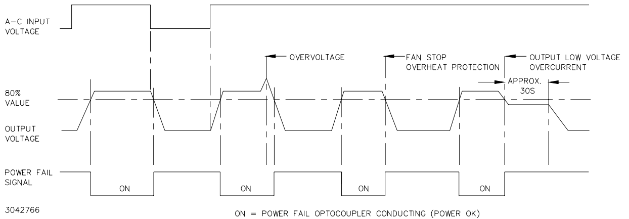
FIGURE 3. RKW 1500W POWER FAILURE TIMING DIAGRAM
