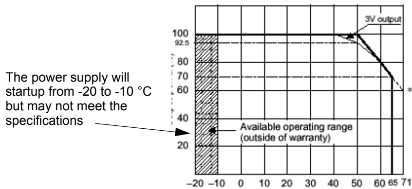
FIGURE 4. POWER RATING VS. TEMPERATURE
