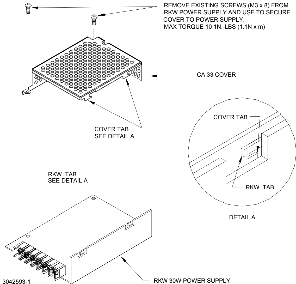
FIGURE 1. CA 33 COVER INSTALLATION
