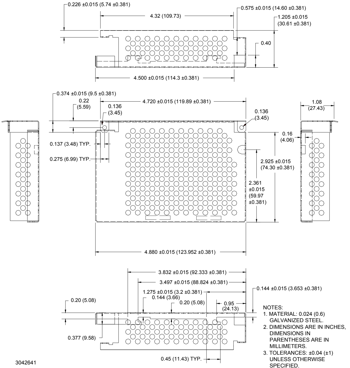
FIGURE 2. CA 33 OUTLINE DIMENSIONS
