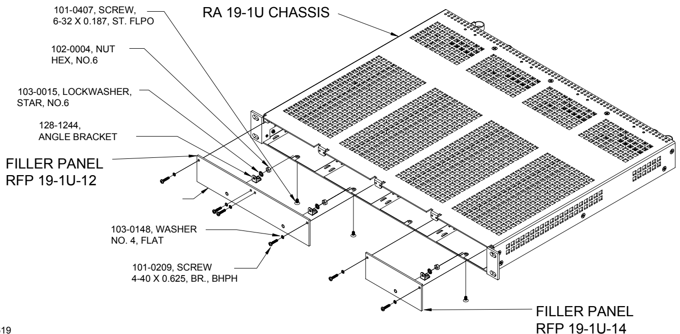
FIGURE 1. FILLER PANEL INSTALLATION
