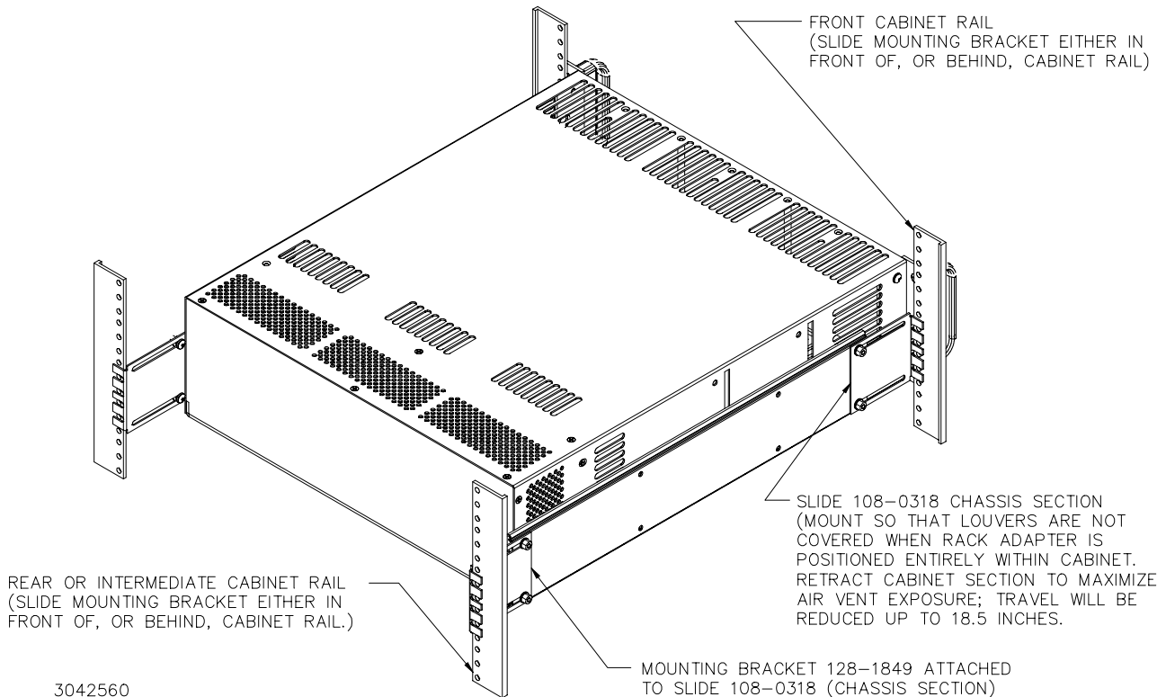
FIGURE 3. ATTACHING CABINET SECTION TO RAIL
