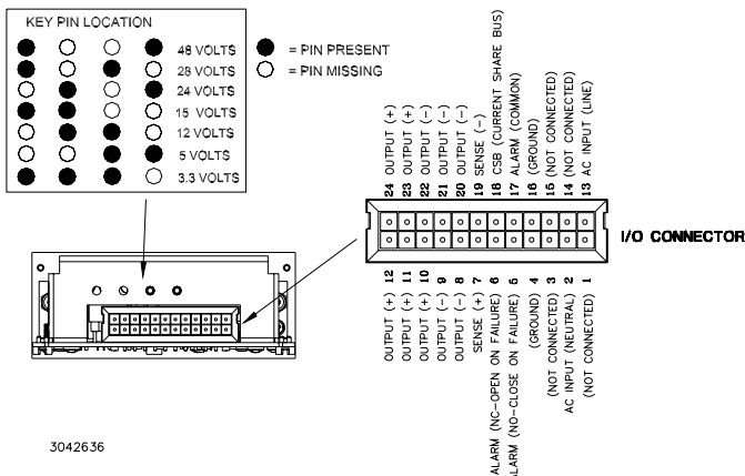
FIGURE 2. REAR CONNECTOR PIN ASSIGNMENTS
