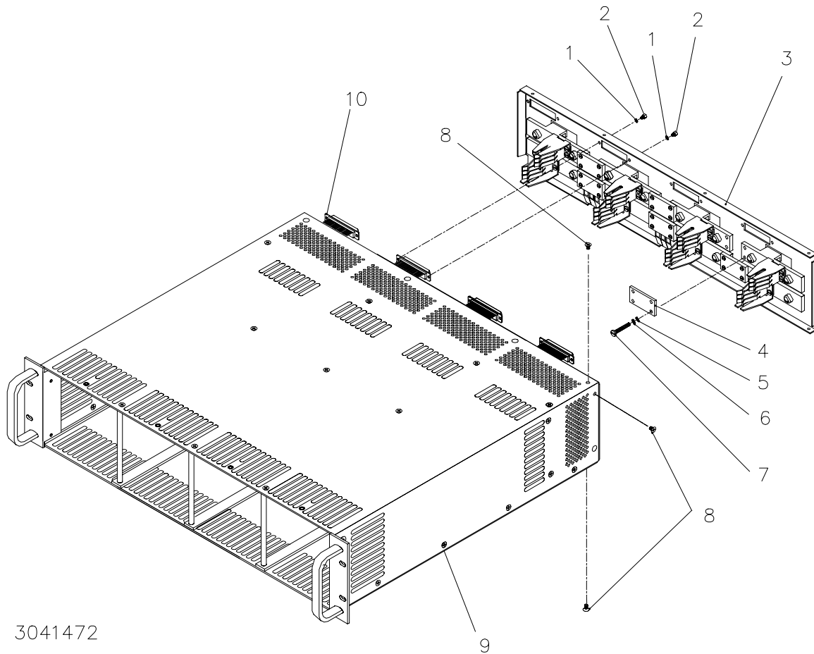
FIGURE 1. BUS BAR LINK REMOVAL/INSTALLATION
