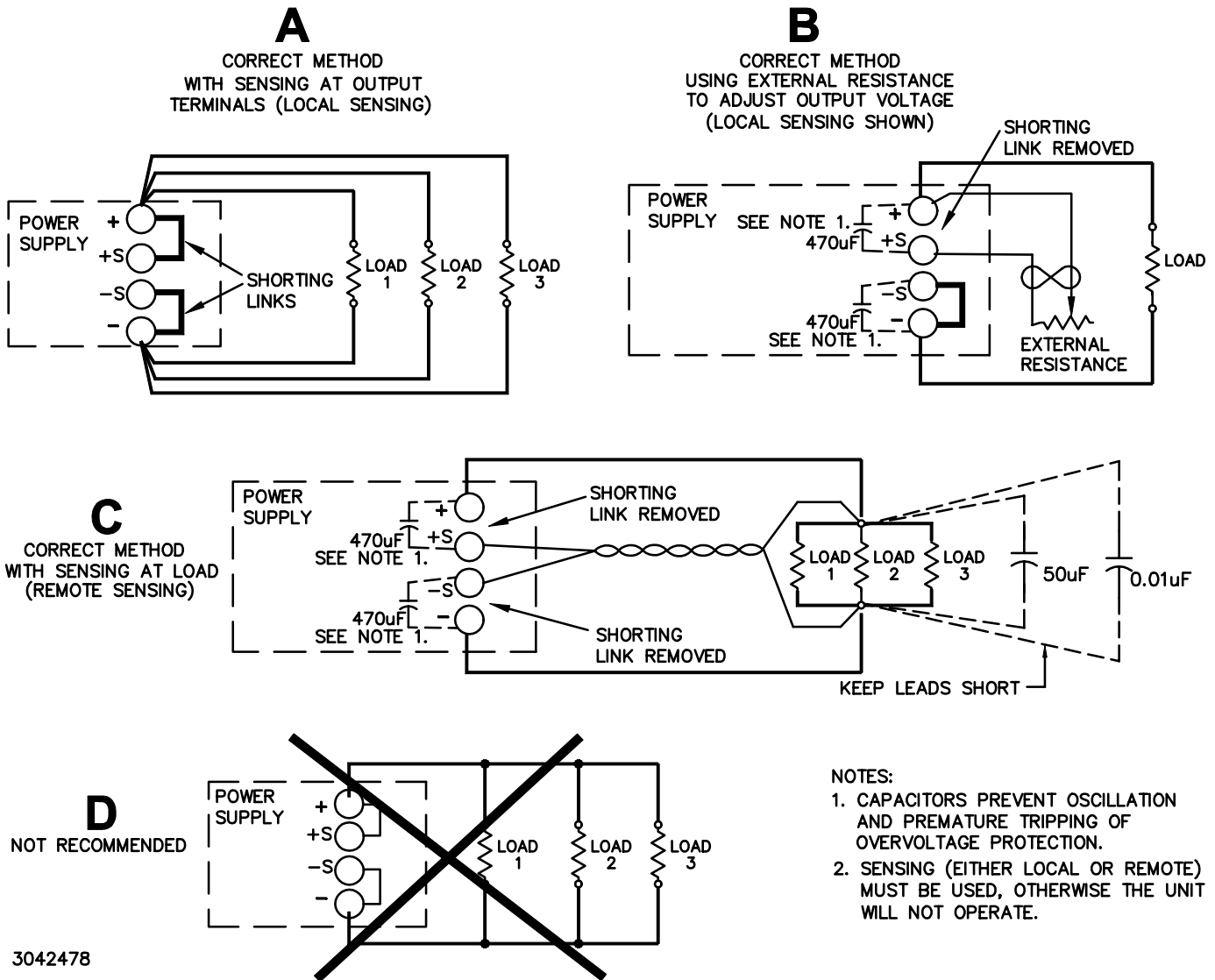
FIGURE 3. LOAD CONNECTIONS
