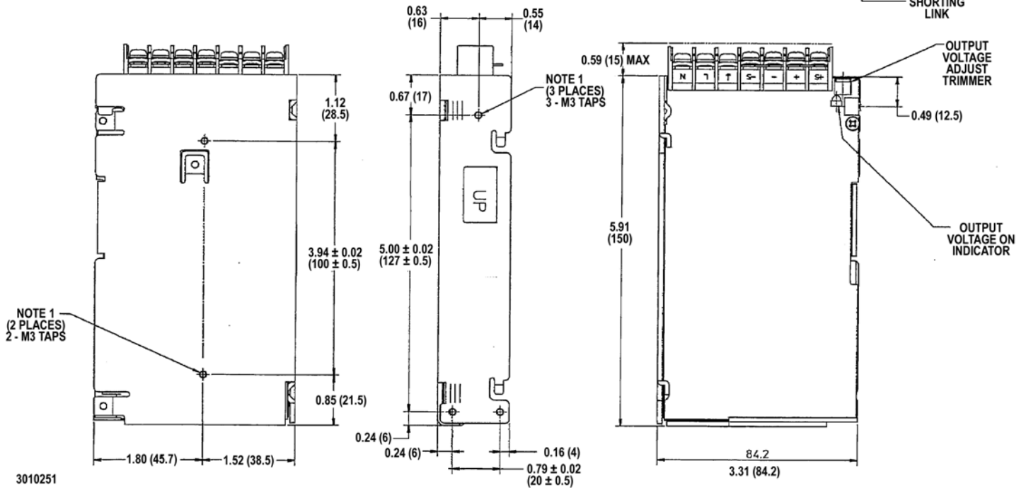
FIGURE 5. RKW 50W MECHANICAL OUTLINE DIAGRAM
