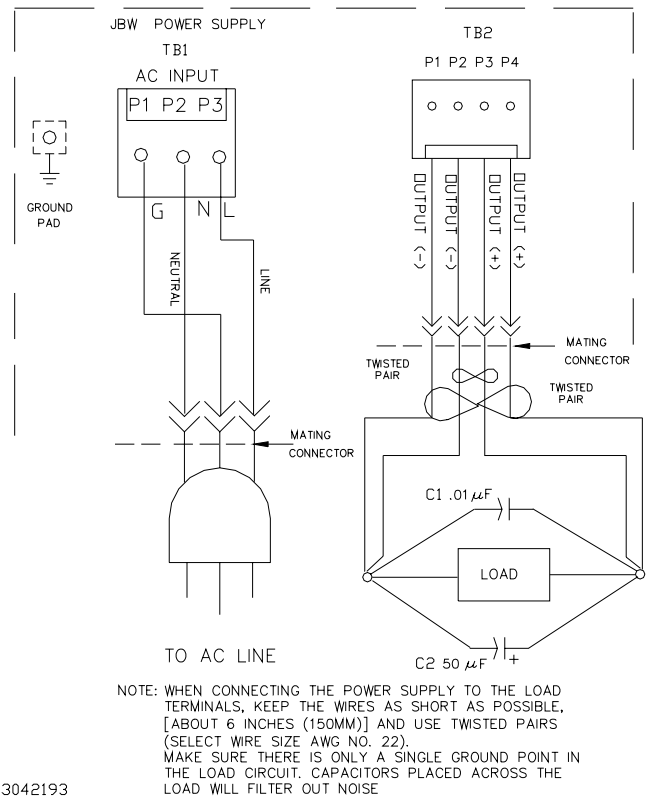
FIGURE 3. LOAD CONNECTIONS
