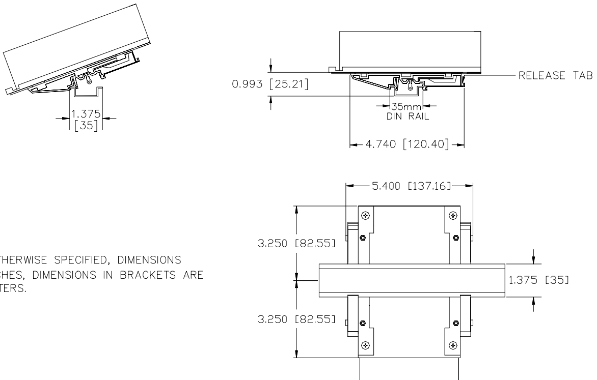
FIGURE 4. MRW POWER SUPPLY WITH KIT INSTALLED, OUTLINE DIMENSIONS
