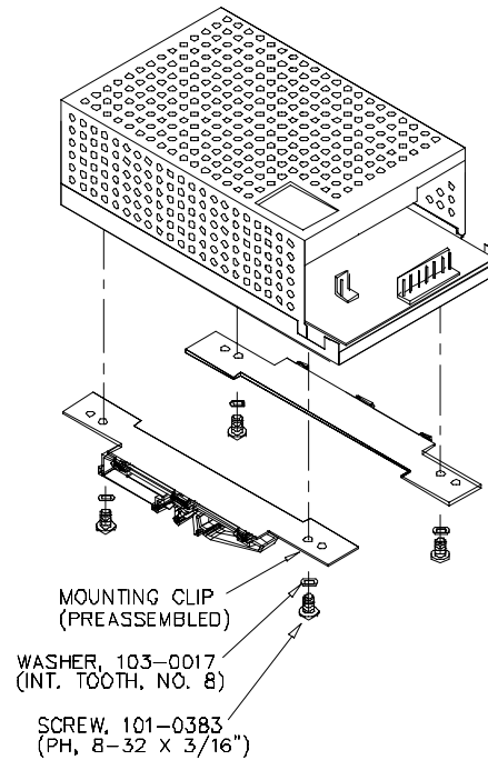
FIGURE 3. INSTALLATION OF KIT ON MRW POWER SUPPLY
