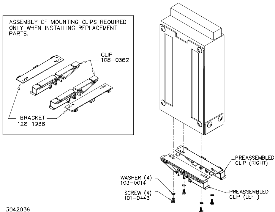
FIGURE 3. INSTALLING CLIPS ON MOUNTING BRACKET
