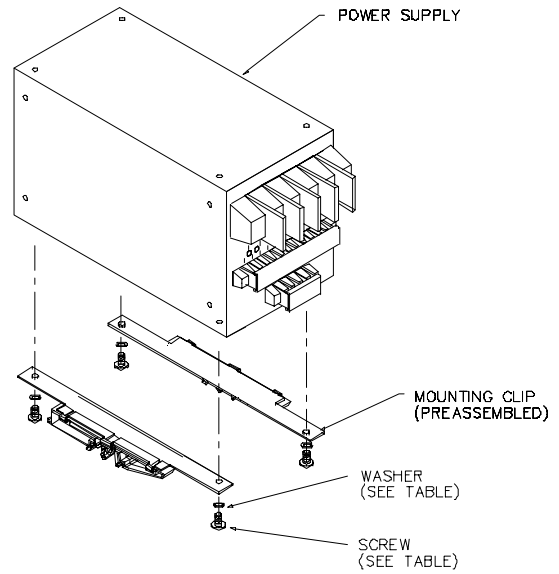
FIGURE 3. INSTALLATION OF KIT ON RAX 175W POWER SUPPLY
