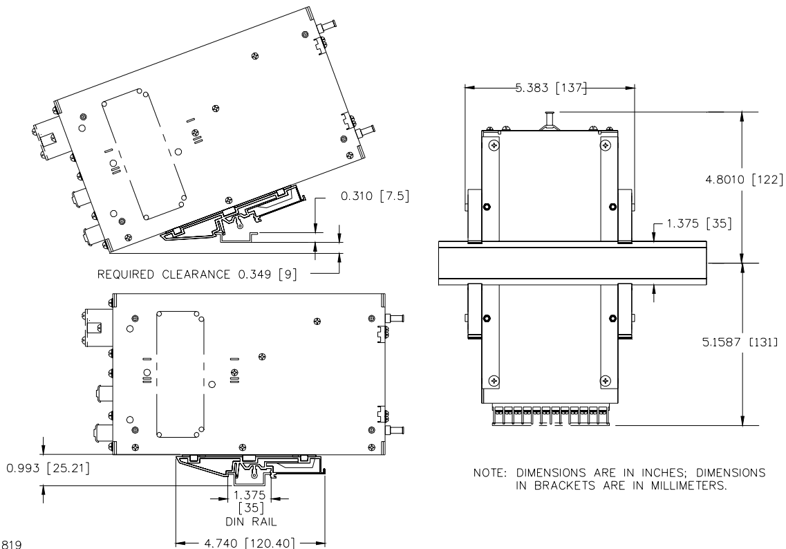
FIGURE 4. RAX 175W POWER SUPPLY WITH KIT INSTALLED, OUTLINE DIMENSIONS
