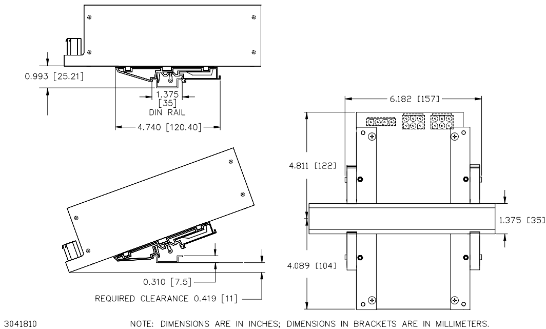
FIGURE 4. POWER SUPPLY WITH KIT INSTALLED, OUTLINE DIMENSIONS
