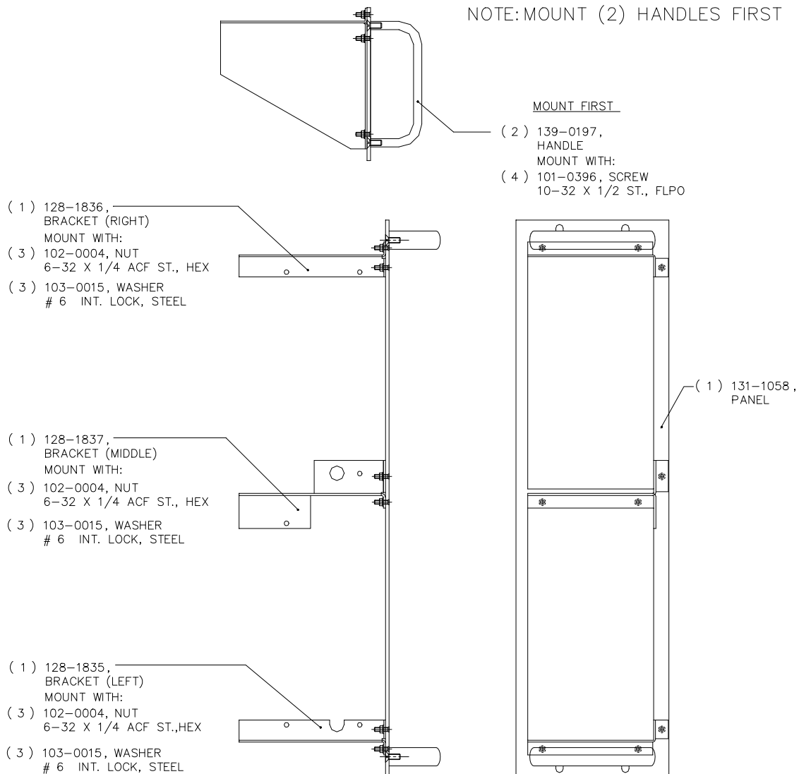
FIGURE 1. RA 72 RACK ADAPTER ASSEMBLY
