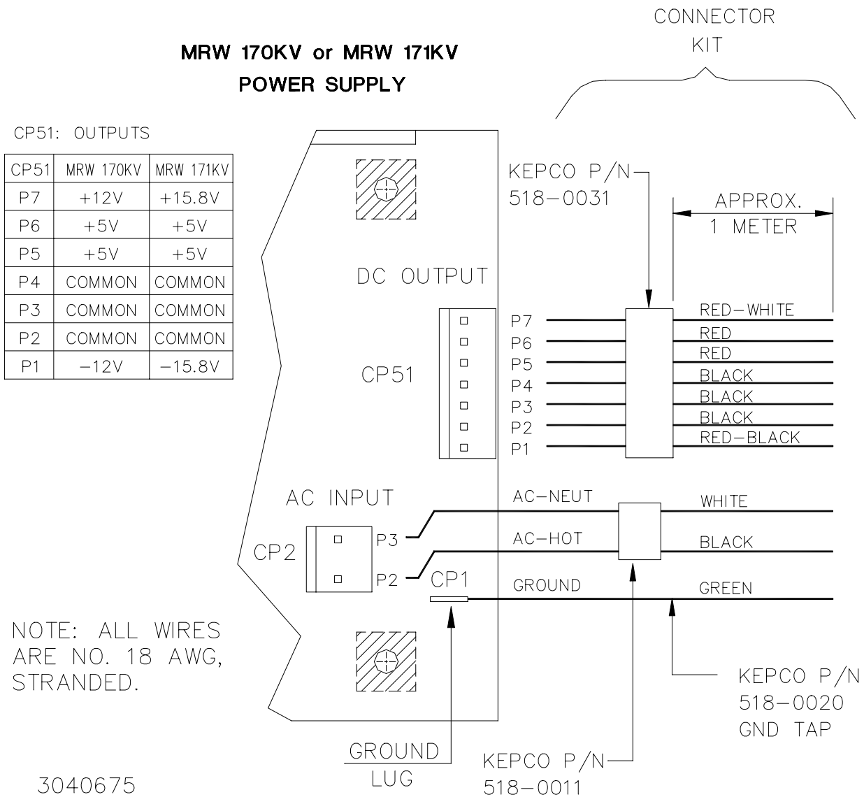
FIGURE 1. CABLE KIT 219-0239
