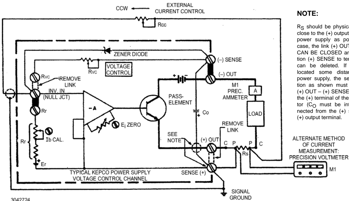
FIGURE 3. CALIBRATION SET-UP
