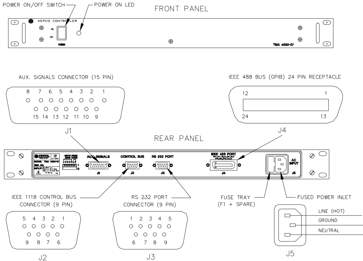
FIGURE 2-2. TMA 4882-27 FRONT AND REAR PANELS
