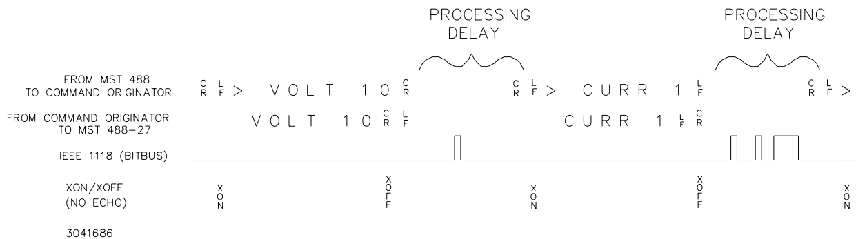
FIGURE 3-1. RS 232 IMPLEMENTATION
