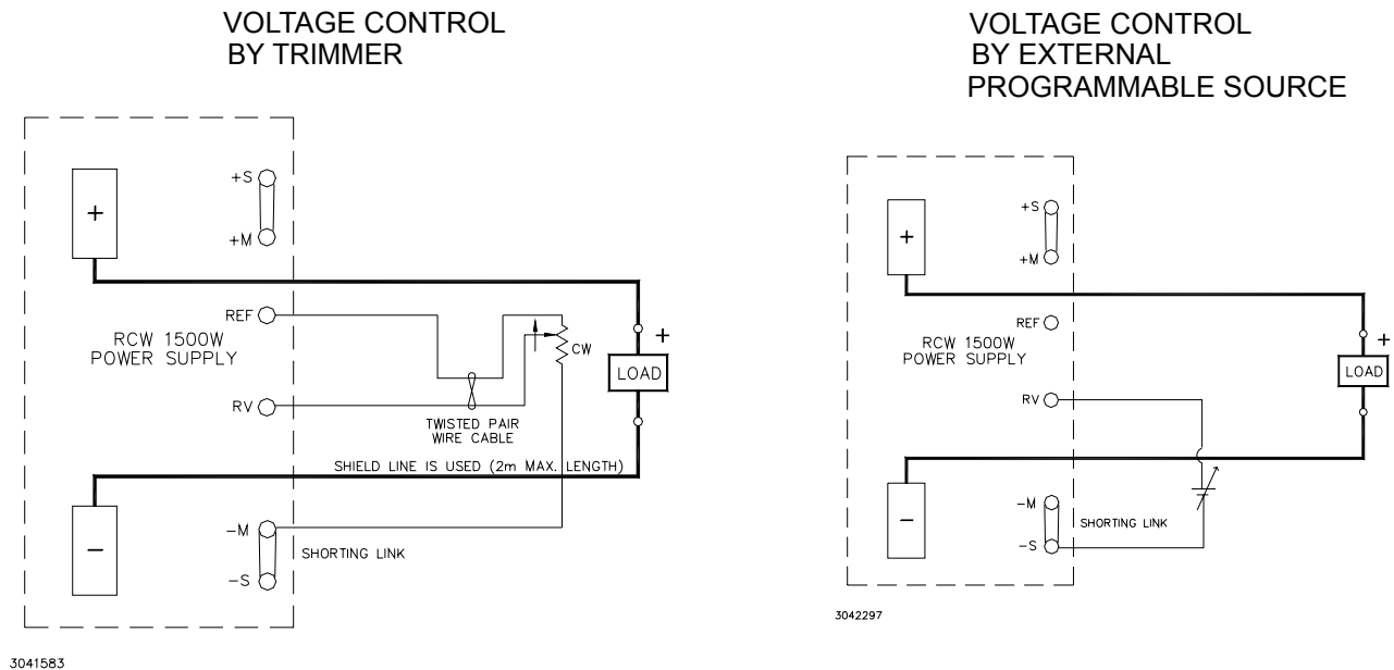
FIGURE 7 CONNECTIONS FOR REMOTE VOLTAGE CONTROL OF THE RCW 1500W POWER SUPPLY
