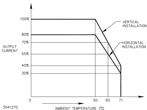
FIGURE 1. TEMPERATURE DERATING
