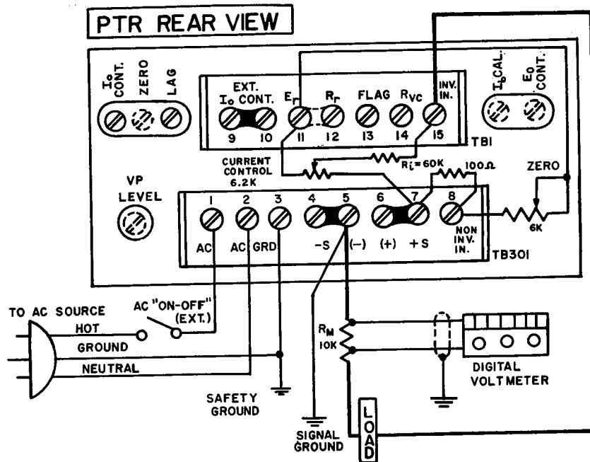
FIG. 3-14 CONNECTIONS FOR CURRENT CONTROL BY VOLTAGE (WITHOUT R_g ).
