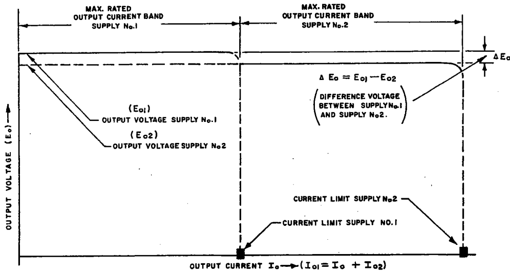
FIG. 3-22 E_o/I_o CHARACTERISTIC OF TWO PARALLEL POWER SUPPLIES.
