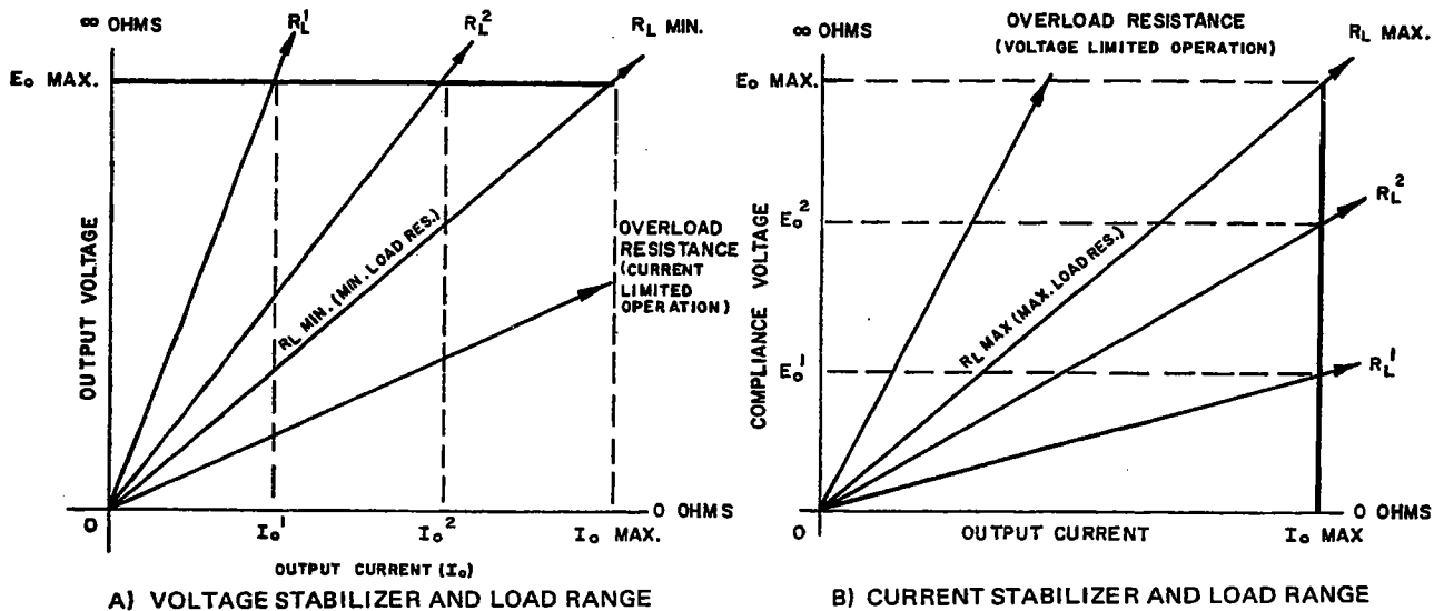
FIG. 3-6 OPERATING CHARACTERISTIC, VOLTAGE VS. CURRENT STABILIZER.
