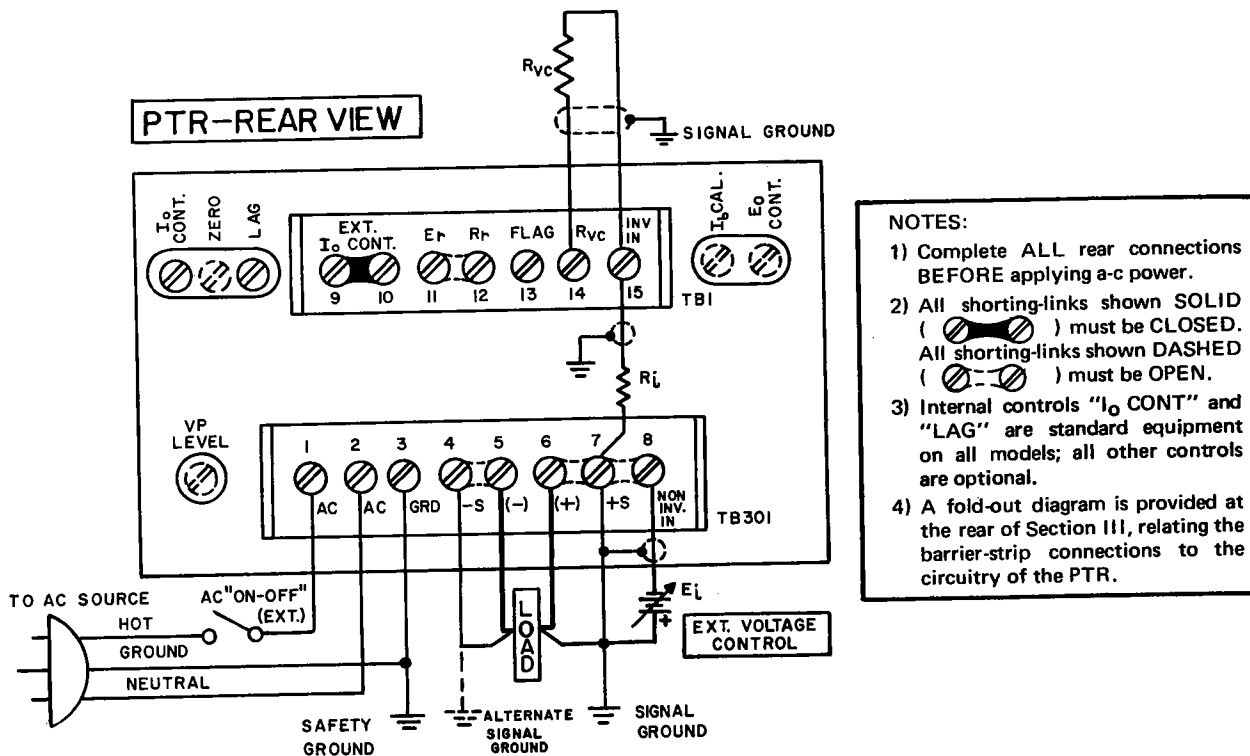
FIG. 3-25 CONNECTIONS FOR NONINVERTING PROGRAMMING.
