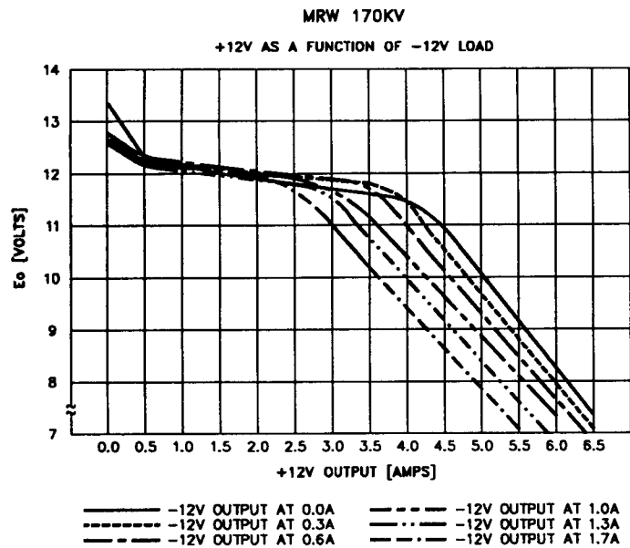
FIGURE 3 +12V OUTPUT AS A FUNCTION OF -12V LOAD (-12V OUTPUT vs. +12V LOAD SIMILAR)
