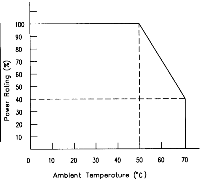
FIGURE 4 PERCENT OUTPUT POWER vs. AMBIENT TEMPERATURE
