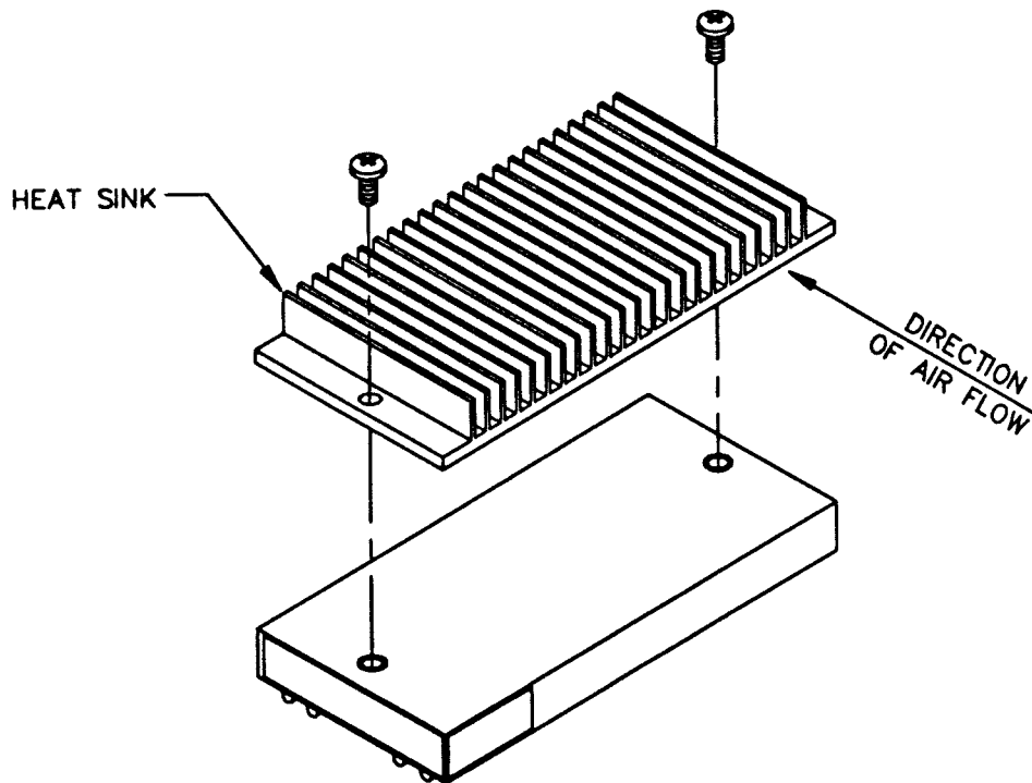
FIGURE 8B HEAT SINK FOR HORIZONTAL MOUNTING OF THE FPD 50-12 DC TO DC CONVERTER
