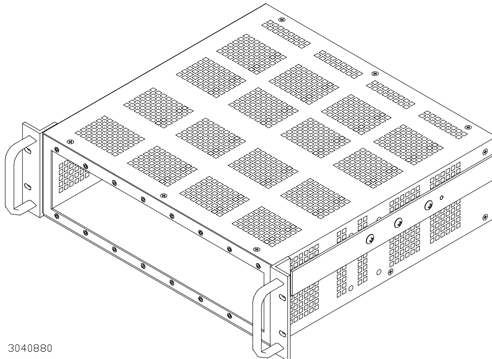
FIGURE 1. KEPCO MODEL RA 44-R RACK ADAPTER
