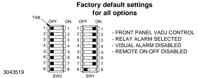
FIGURE 1. DIP SWITCH FACTORY DEFAULTS
