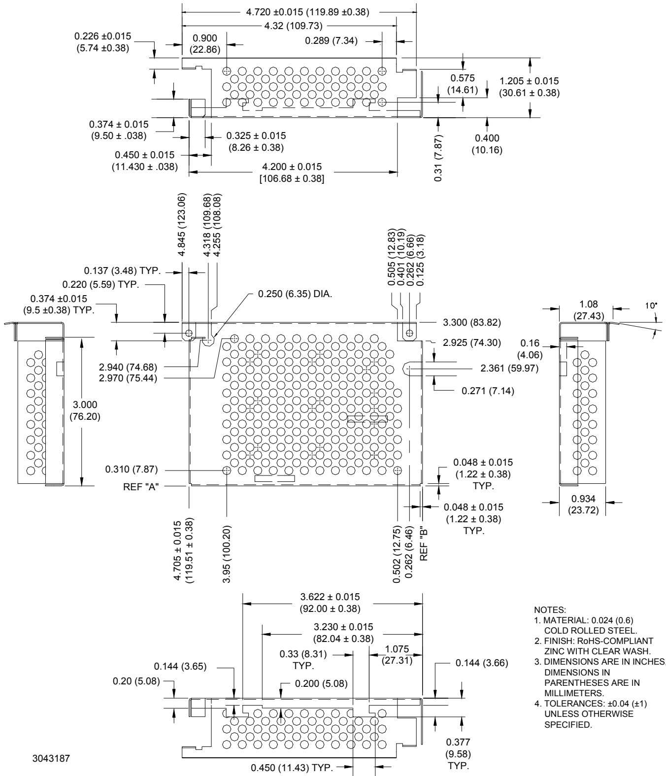
FIGURE 2. CA 33-R OUTLINE DIMENSIONS
