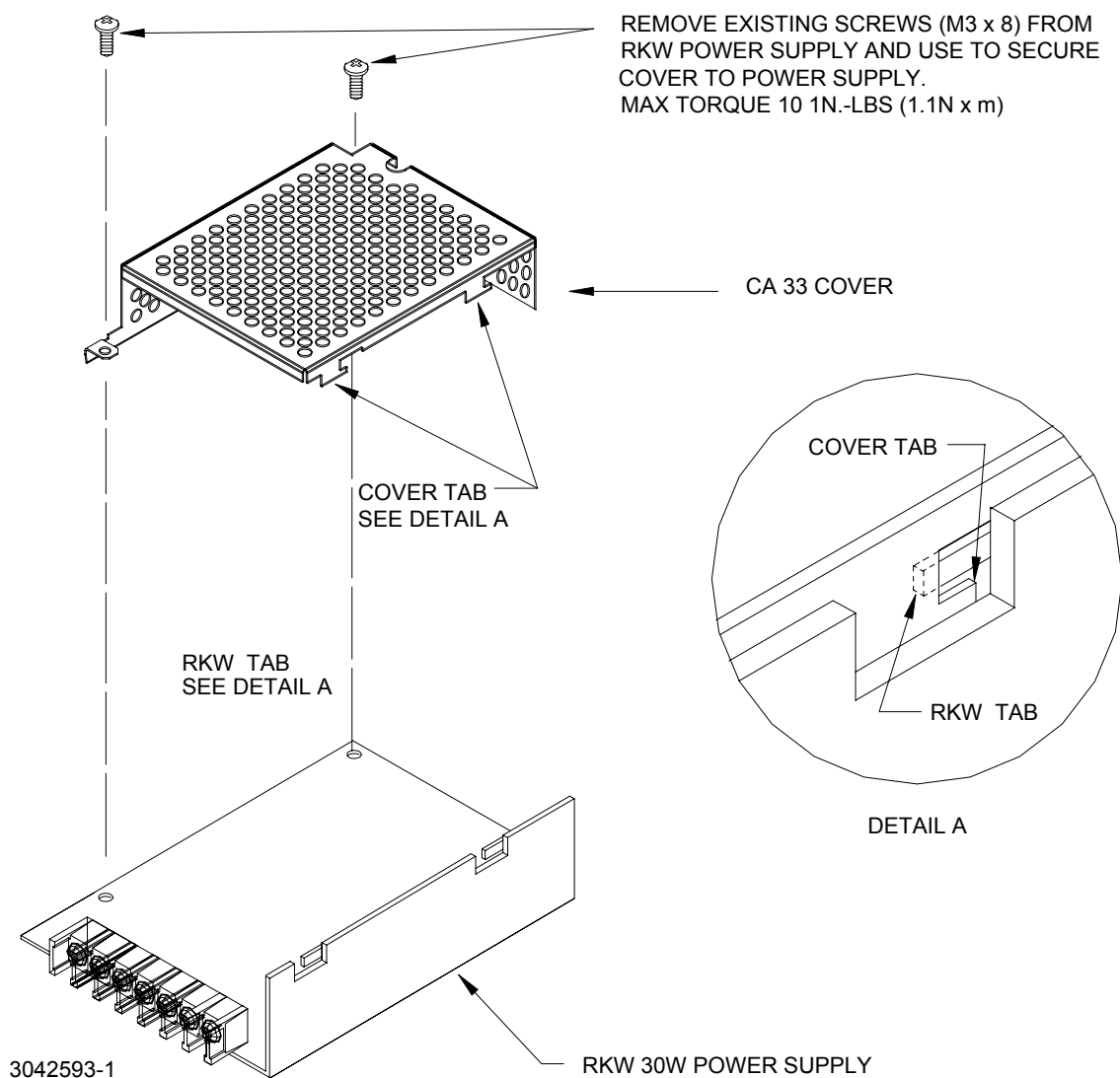
FIGURE 1. CA 33-R COVER INSTALLATION
