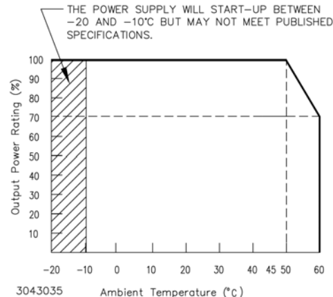
FIGURE 1. DERATING PLOT
