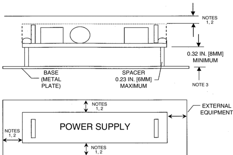
FIGURE 2. MOUNTING DIRECTION
