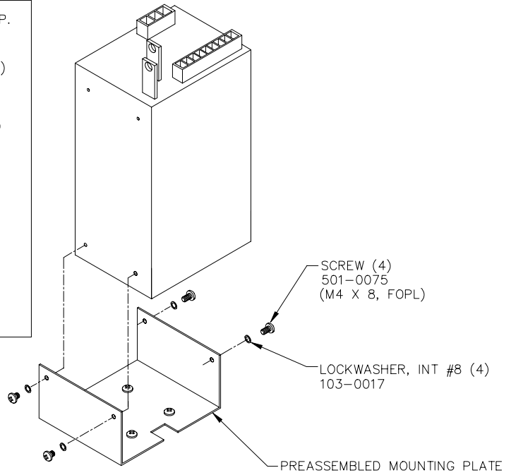
FIGURE 3. INSTALLATION OF KIT ON RKW 600W POWER SUPPLY
