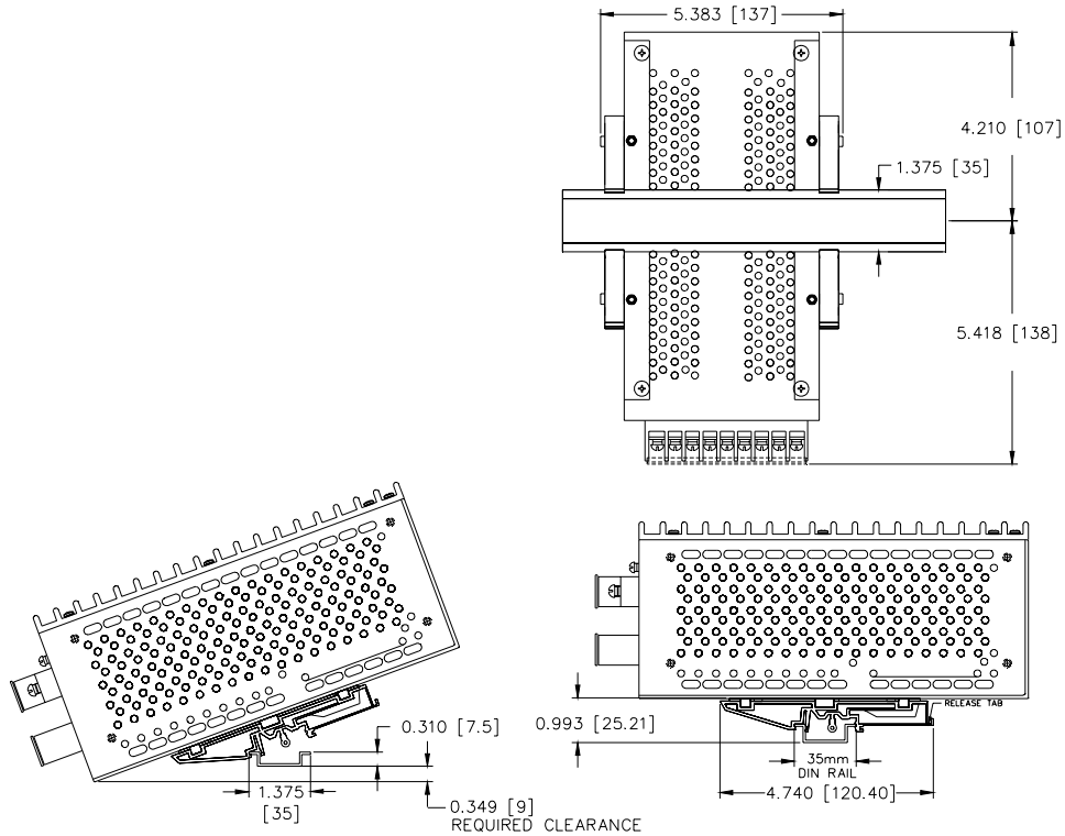
FIGURE 4. RCW 175W POWER SUPPLY WITH KIT INSTALLED, OUTLINE DIMENSIONS
